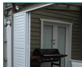
d. Fit shutter panels, inserting top into upper channel first.
